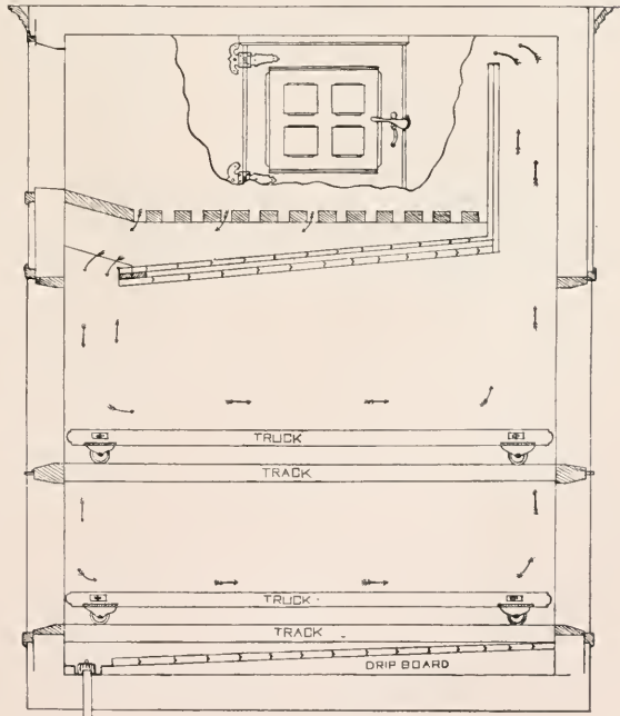
FIG. 8.—Cross-section.
